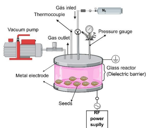
Figure 1 - (A) Schematic of the experimental setup used to treat 'Carrizo' citrange seeds with nitrogen plasma; (B) Photograph of the reactor under operating conditions
