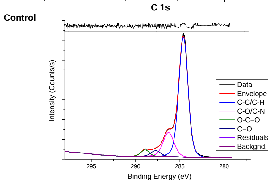
Figure 4 - X-ray photoelectron spectroscopy (XPS) spectra of untreated 'Carrizo' citrange seeds (control) and after nitrogen plasma treatment, treatment time of 1, 2 and 3 min, with 30 W power.
